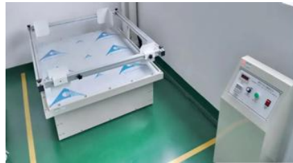
Transportation Vibration Test Machine
